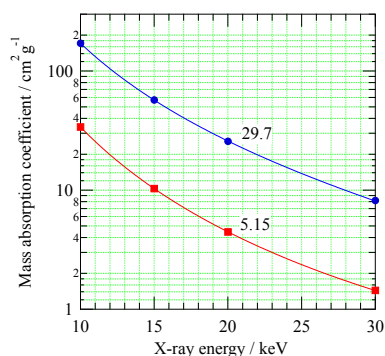
Figure 1. Mass absorption coefficient as a function of X-ray energy.
